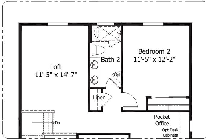
Opt. 2-Bedroom with Loft Upper Level Layout
