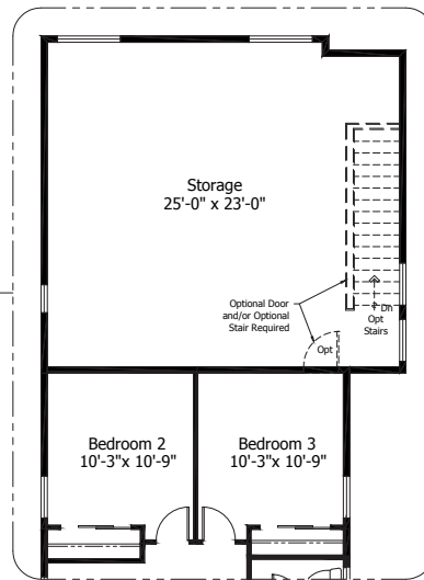
OPTIONAL STORAGE (SHOWN W/ OPT STAIRS TO GARAGE)
