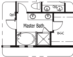
Optional Master Bathroom Layout w/ "Soaker" Tub
