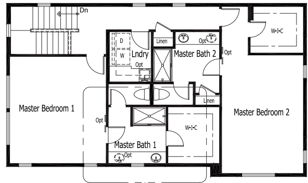
Optional Double Master Bedroom Layout
