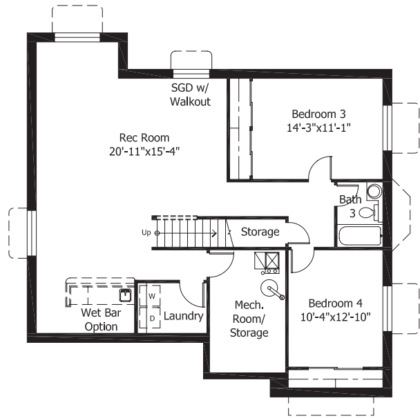
Basement Level With Optional Finish
